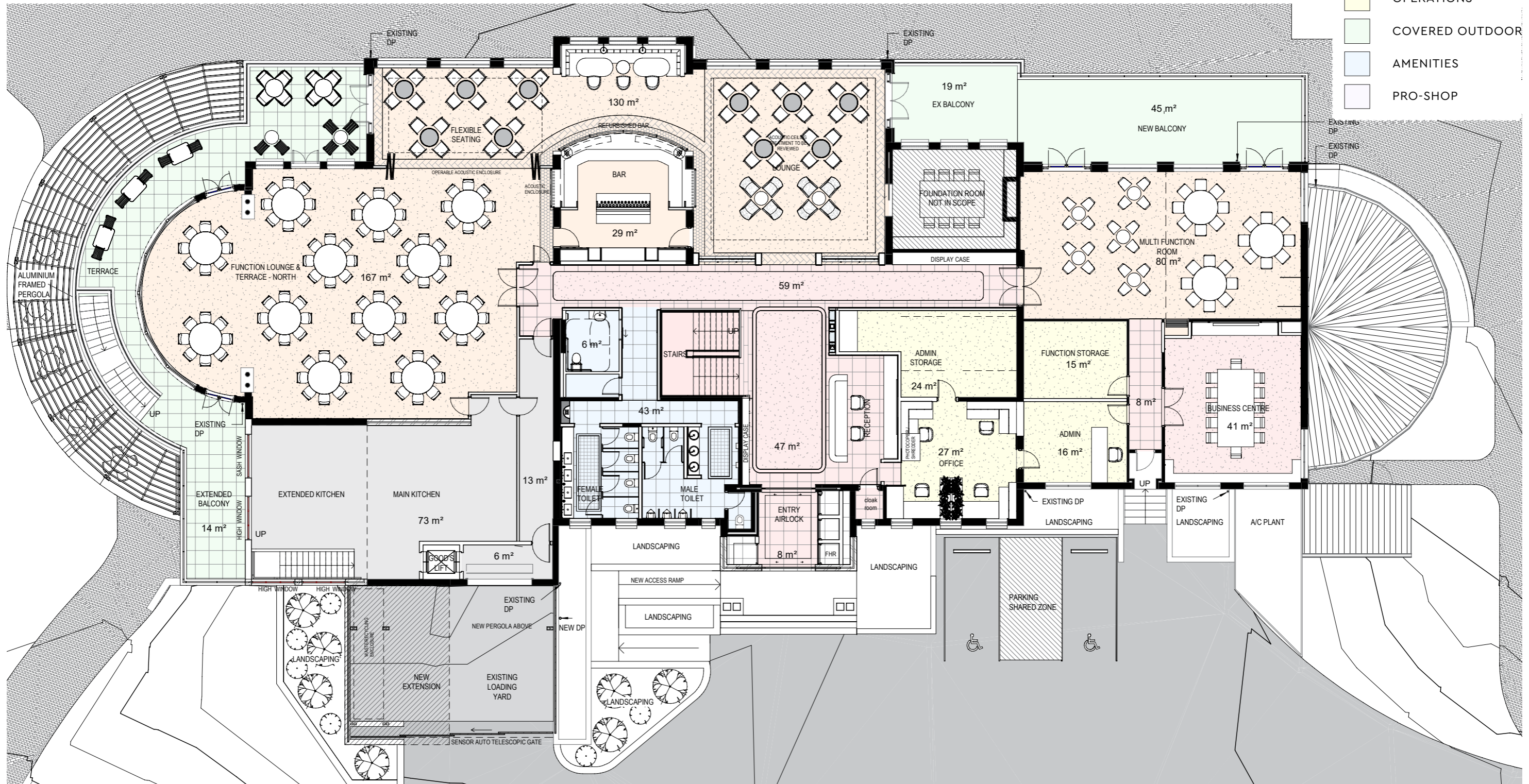
GF FLOOR PLAN VIEW
