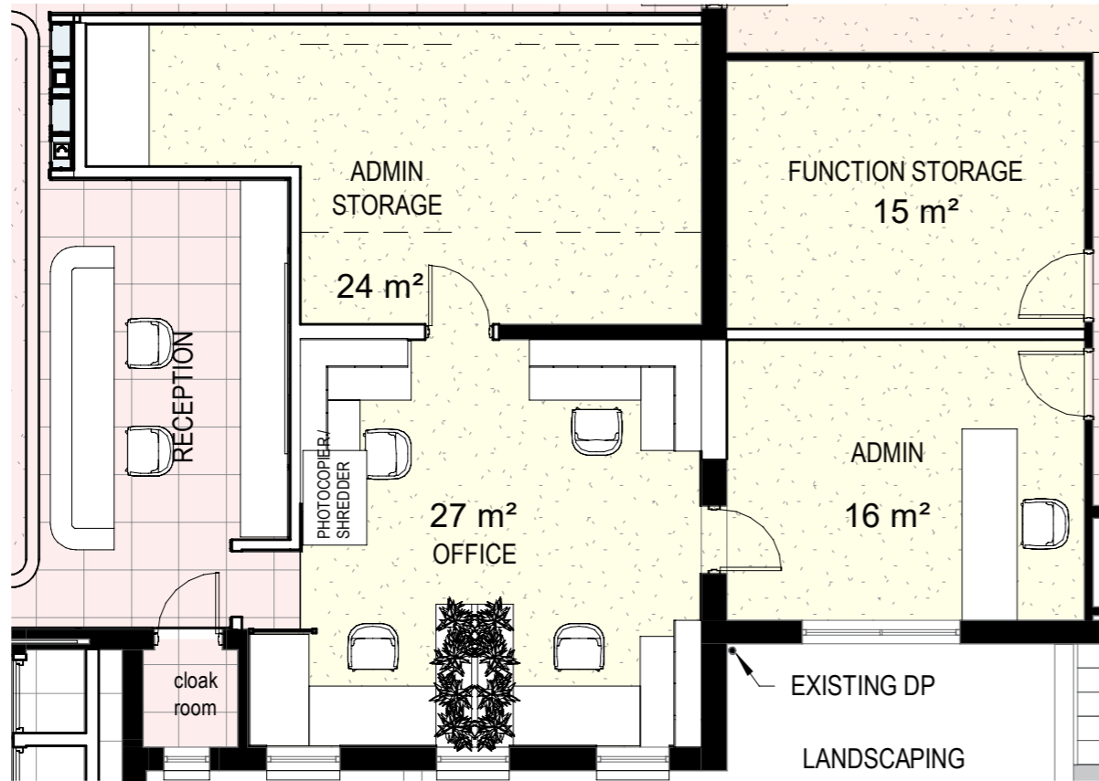
DETAIL PLAN VIEW GF
