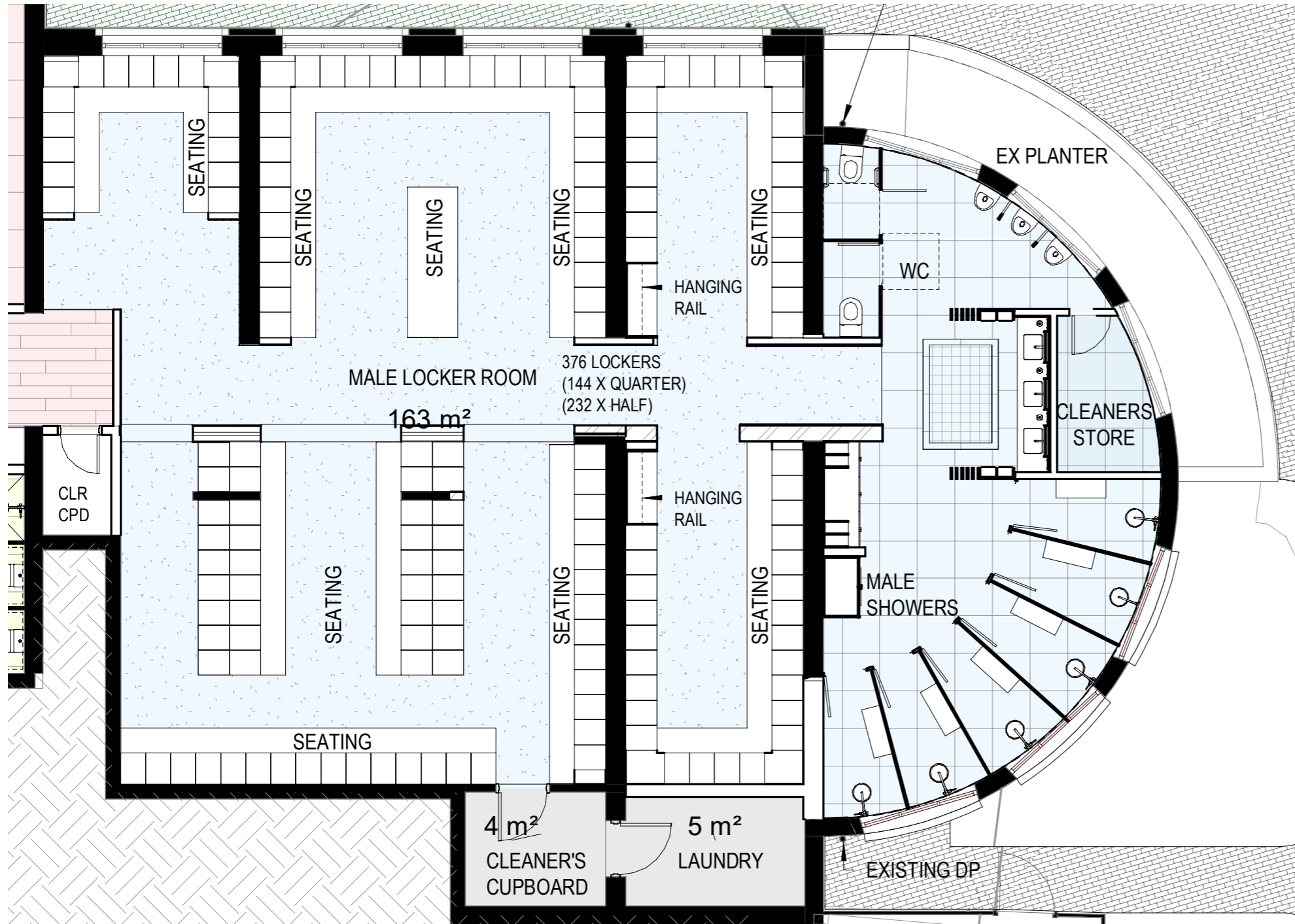
DETAIL PLAN VIEW
