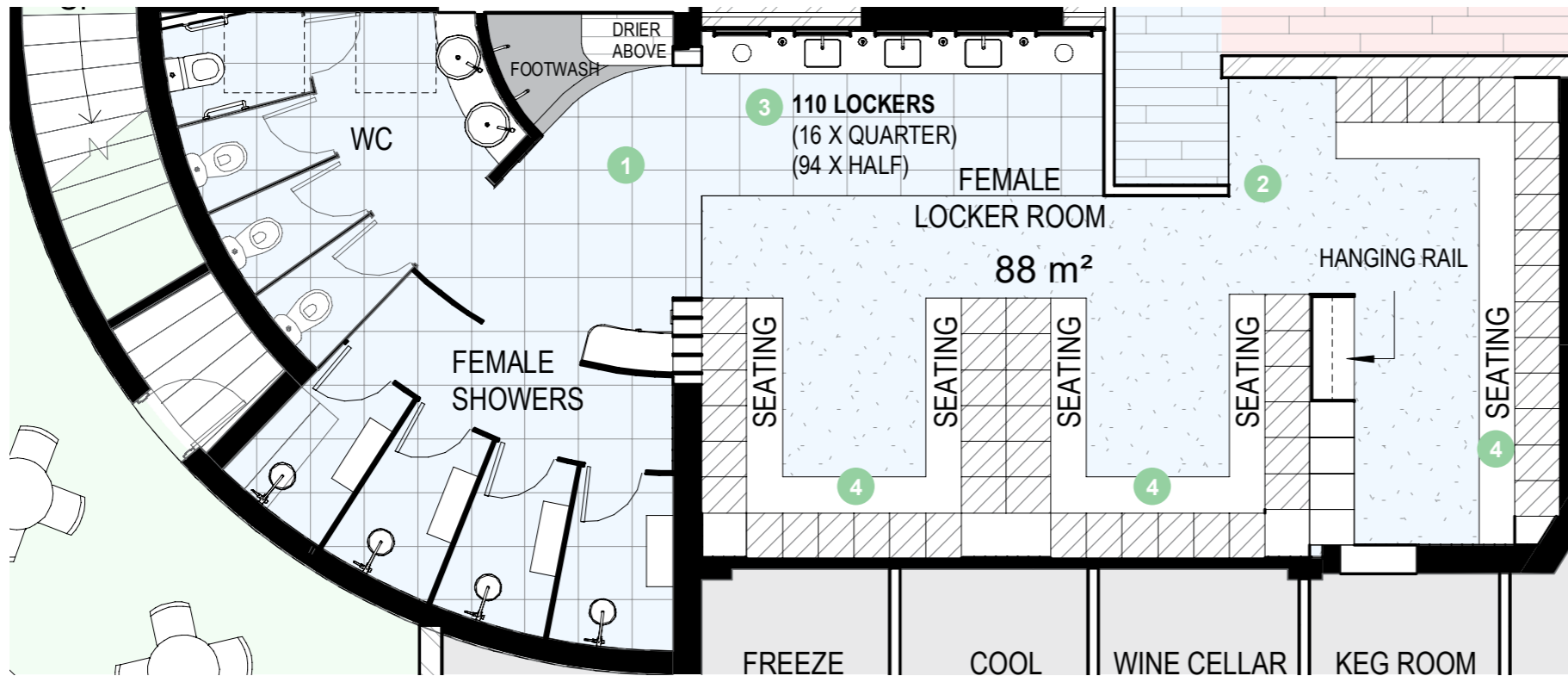
DETAIL PLAN VIEW
